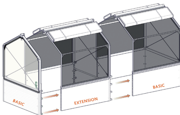
FC3020 + FC3040 GrowCamp BASIC + EXTENSION
